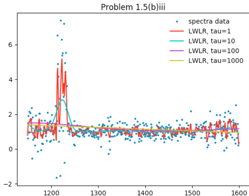
Figure 4: The first row of quasar spectra data plotted against wavelengths along with the curves resulting from locally weighted linear regressions with \tau = 1, 10, 100 , and 1000.
